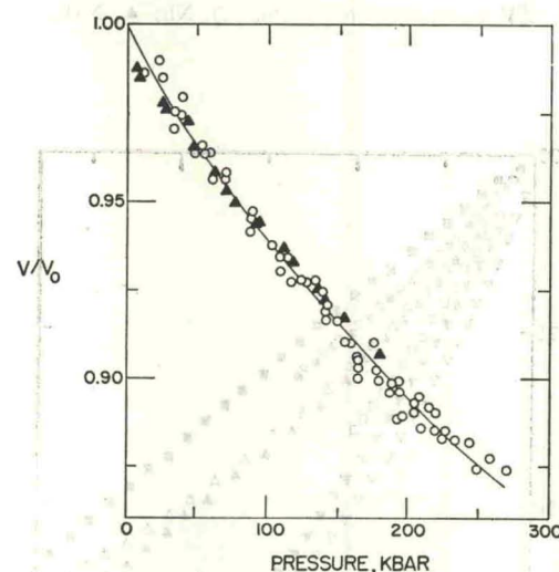
FIG. 1. V/V_0 vs pressure—Fe 3 Al. (O, Nb; ▲, NaCl.)
